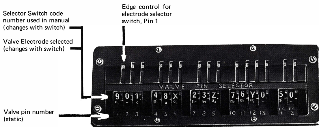
Top view of the barrel switch assembly on an AVO VCM 163. Other tester models are similar, but some have fewer switch rollers
