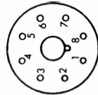
International Octal (A08)
