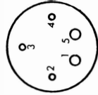
American 5 pin (UX5)
