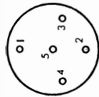
British 4/5 Pin (B5 & 4)
